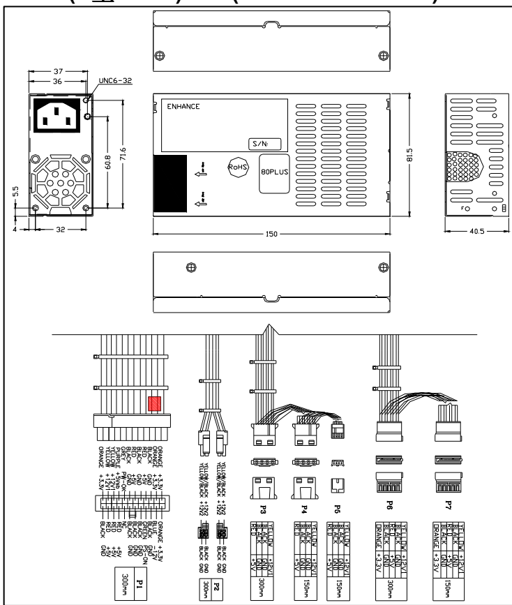
(B型CASE)Dim (L150*W81.5*H40.5)
