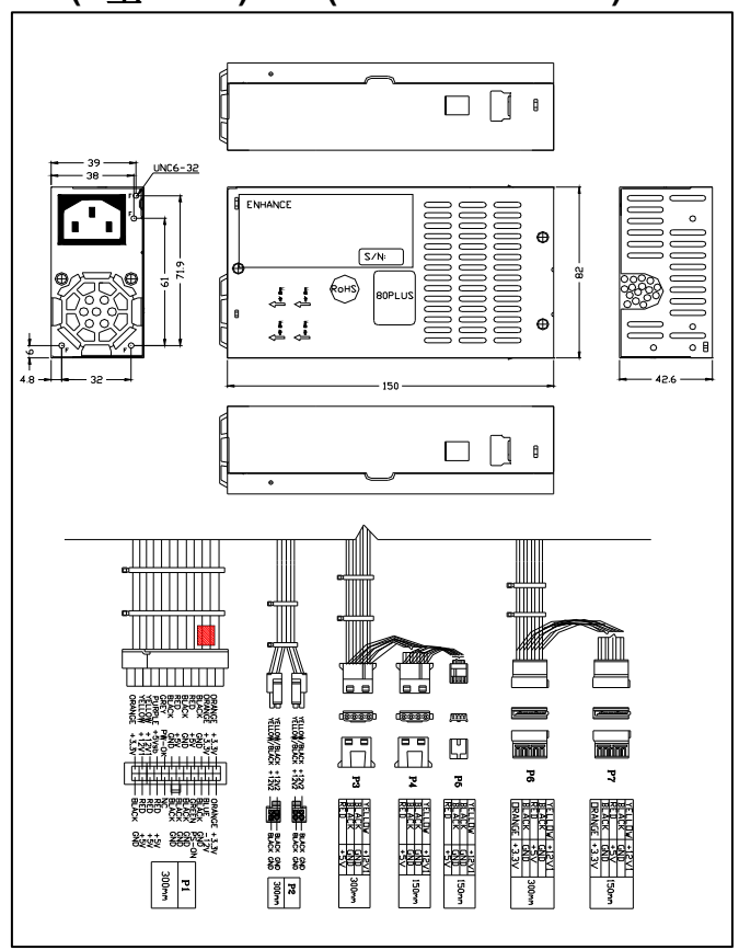
(C型CASE)Dim (L150*W82*H42.6)
